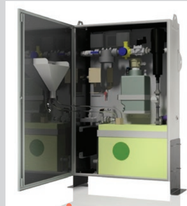
ProMix release agent mixing system
